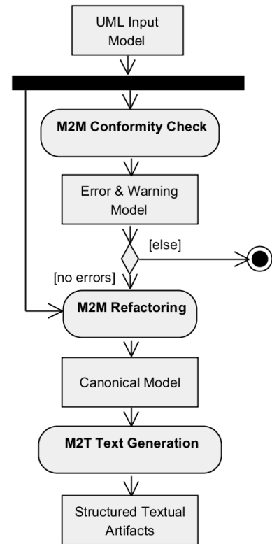
Figure 1: MeDMT Transformation Architecture
